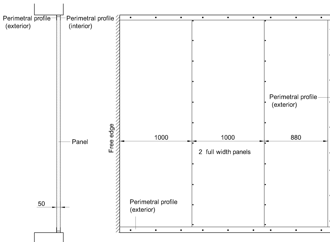
Figure 1 – Test setup (dimensions in mm)
