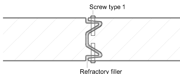
Figure 4 – Joint between panels
