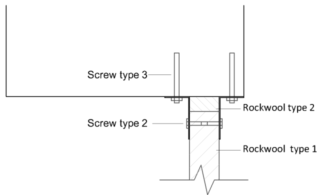
Figure 3 – Perimetral fixation of the specimen
